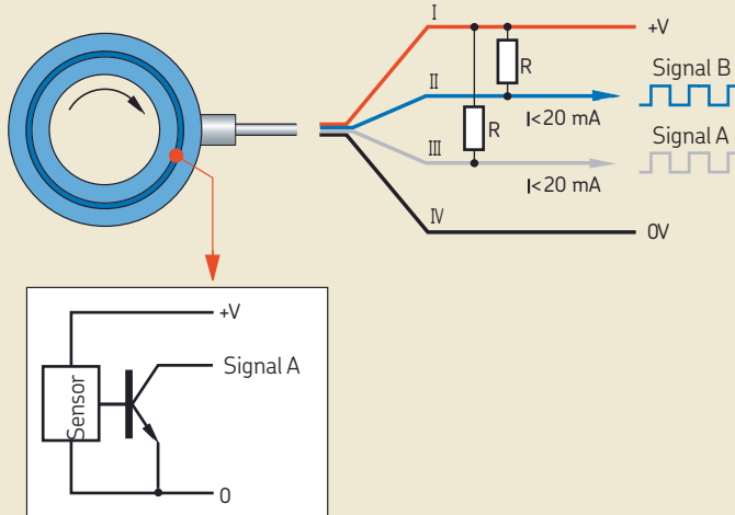
Circuit diagram
