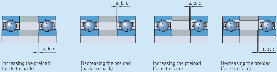
Guideline values for spacer ring width reduction – 72 .. D bearing series
