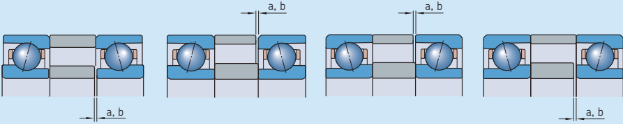
Guideline values for spacer ring width reduction – 719 .. E and 70 .. E bearing series
