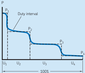
Histogram of constant load blocks
